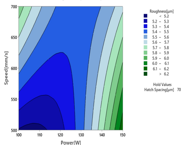
Contour Plot of Roughness[ \mu\text{m} ] vs Speed[mm/s], Power[W]
